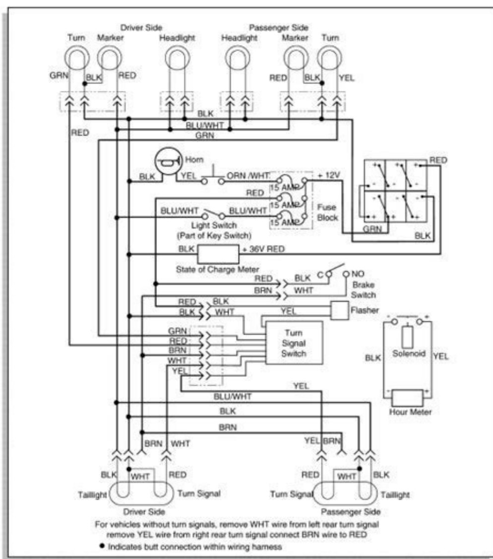
Fig. 2 Accessory Wiring Diagram
